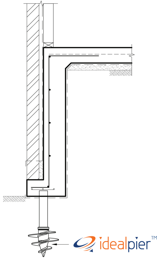
TYPICAL DROPPED EDGE BEAM DETAIL
